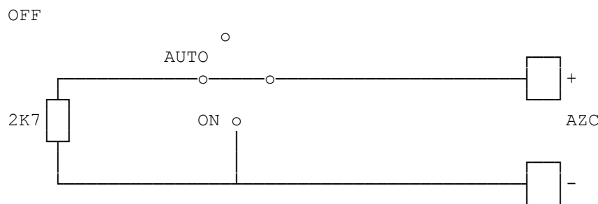
B. WITH A ROTARY SWITCH, "ON" IS B1 (INSTANT), "OFF" IS FAULT.
